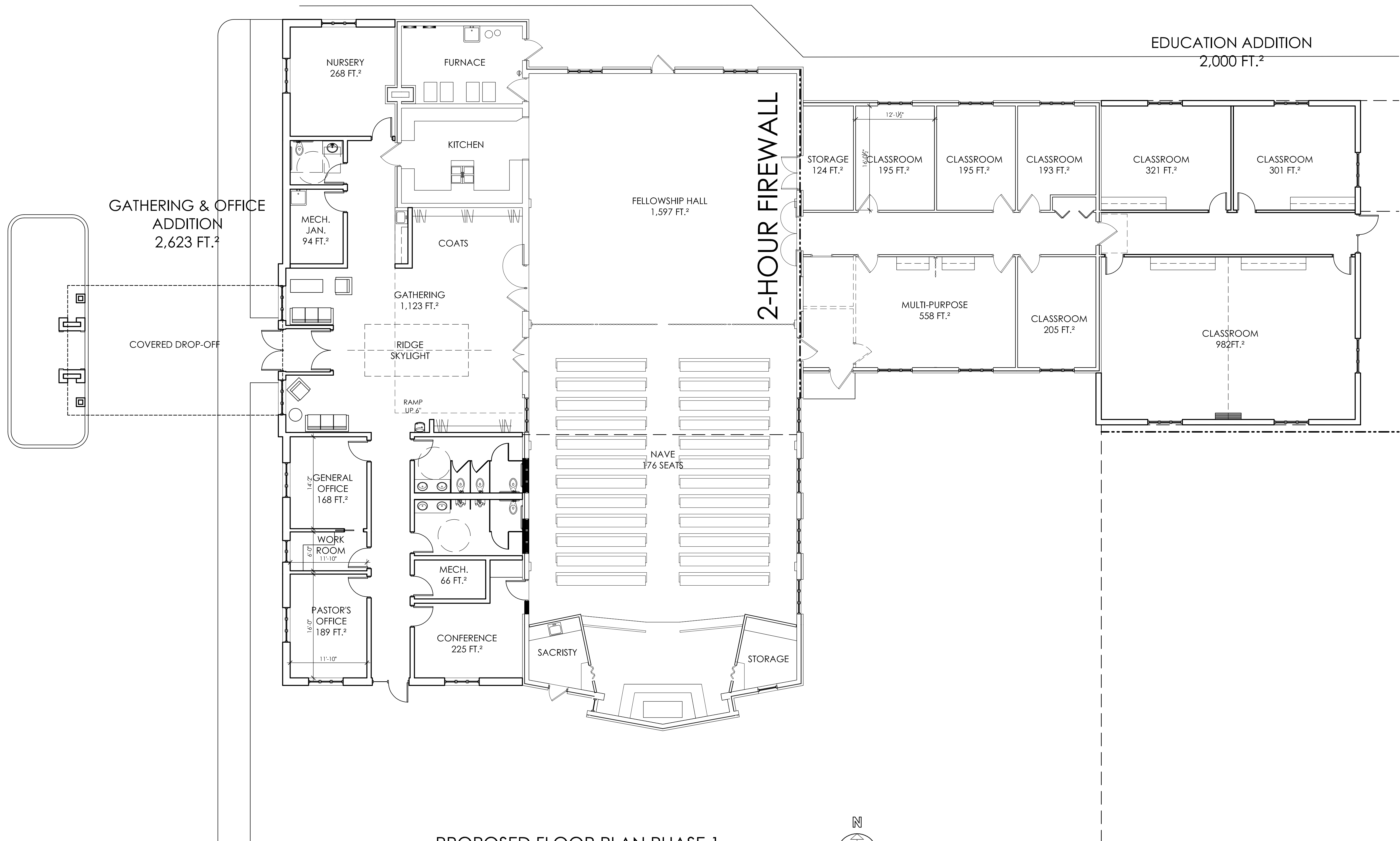
PROPOSED FLOOR PLAN PHASE 1
